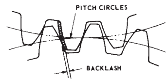
FIGURE 1.12 — BACKLASH
