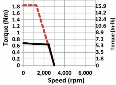
J0400-4x4-4-000(400 Watts) -10Amps DC Bus--24VDC
