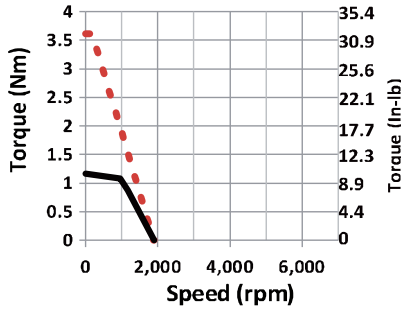
J0300-4x4-5-000(300 Watts) -10Amps DC Bus--24VDC
