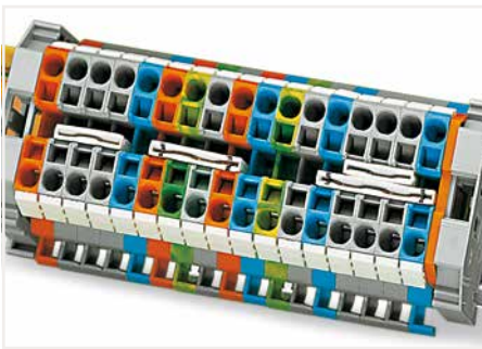
Commoning with push-in type jumper bars: Two parallel jumper slots are accommodated in one terminal block.
