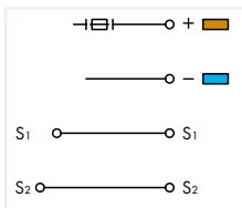
Sensor LED terminal block; for fuse plugs; for PNP (high-side) switching sensors; with gray end plate Terminal block width: 6 mm / 0.236 inch
