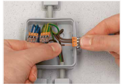
Termination: Insert the stripped solid conductor until it hits backstop.
