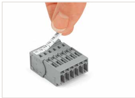
Labeling a male connector with CAGE CLAMP® connection via Mini-USB Quick Markers.
