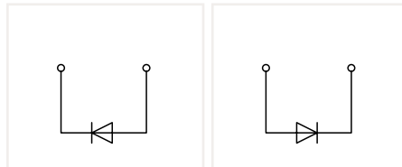
2-pin diode carrier terminal block; with two jumper positions
