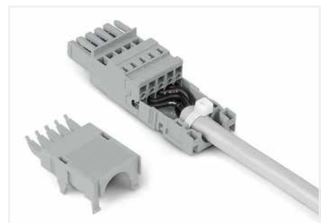
2- to 5-pole strain relief housings feature one cable outlet (rear side). 6- to 9-pole strain relief housings feature two cable outlets and one cover. 10- to 16-pole strain relief housings feature three cable outlets and two covers.
