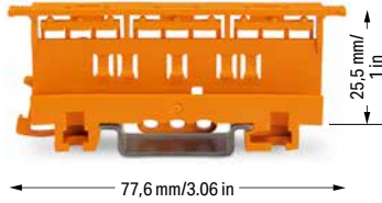
Mounting carrier; for 2-, 3- and 5-wire splicing connectors (4 mm 2 ); 17.5 mm wide
