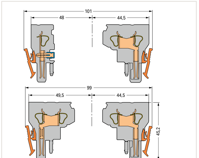
2 x 2-conductor female plugs Carrier terminal blocks can be commoned via 280 and 780 Series Jumpers and tested using a test plug adapter (280-4..).
