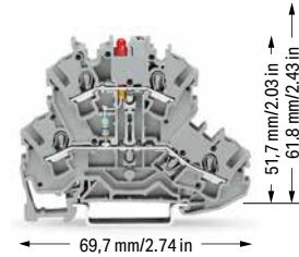
2002-2221/1000-434 2002-2221/1000-413
