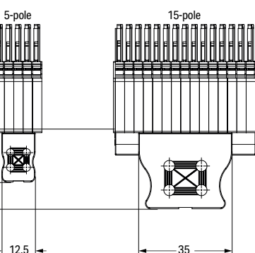
Dimensions of strain relief plates
