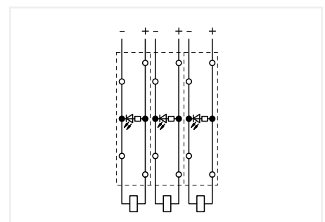
Circuit-related voltage indications can be created using the following terminal blocks: 2002-2221/1000-434 or 2002-2221/1000-413
