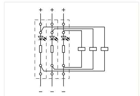
Circuit-related voltage indications can be created using the following terminal blocks: 2001-1421/1000-434 or 2001-1421/1000-413
