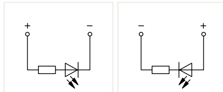
2-pin LED carrier terminal block; with two jumper positions
