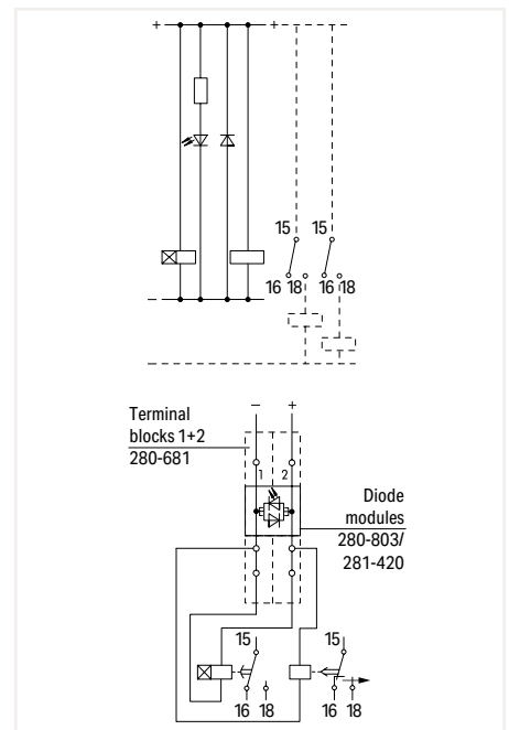
Free-wheeling diode and voltage check
