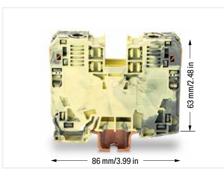
2-conductor through terminal block, dark gray/yellow (285-131), for ground connection without contact to the DIN-rail
