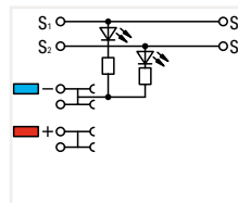
3-conductor sensor terminal block; yellow LED; for PNP (high-side) switching sensors
