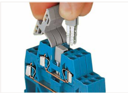
Commoning using an adjacent jumper (280-402). push jumpers down until fully inserted.
