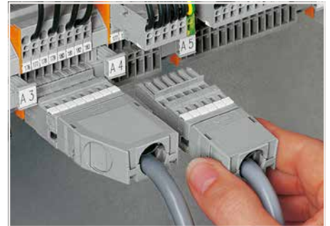
Application: Snap-on type strain relief housings for 769 Series
