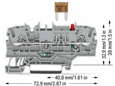
2002-1981/1000-414
