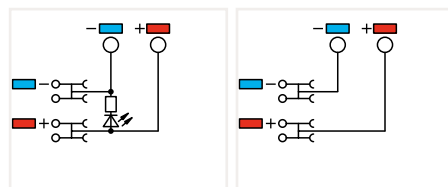
3-conductor sensor LED supply terminal block; green LED; 24 VDC control panel side: 2.5 (4) mm 2 ; max. 28 A
