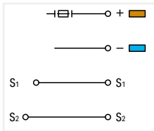
Sensor LED terminal block; for fuse plugs; for PNP (high-side) switching sensors; without end plate
