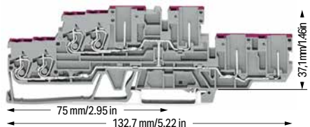
4-conductor/4-pin double-deck carrier terminal block; 4-conductor/4-pin through terminal block; internally commoned; Violet conductor entry; Gray housing
