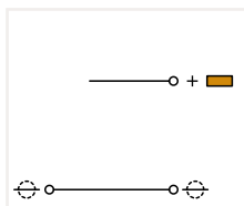
Actuator supply terminal block; with shield connection; power supply from control panel side; with end plate Terminal block width: 6 mm / 0.236 inch
