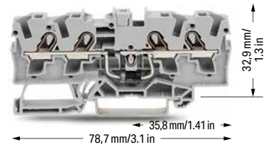
2004-1411/1000-401 2004-1411/1000-400
