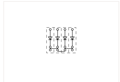
Polarized diode gates with a common cathode can be created using the following terminal blocks: 281-673/281-400 or 281-673/281-401
