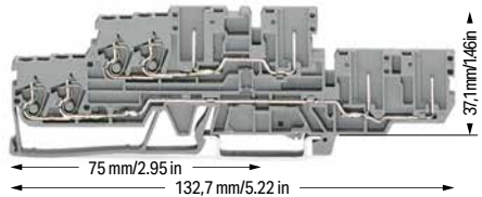
2-conductor/2-pin double-deck carrier terminal block; Through/through terminal block; Gray housing
