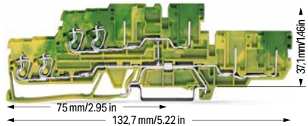
4-conductor/4-pin double-deck carrier block; 4-conductor/4-pin ground conductor block; internally commoned; Green-yellow housing
