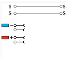
3-conductor sensor terminal block
