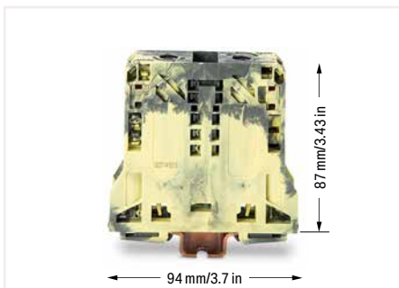
2-conductor through terminal block, dark gray/yellow (285-151), for ground connection without contact to the DIN-rail
