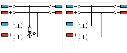
3-conductor sensor LED supply terminal block; green LED; 24 VDC
