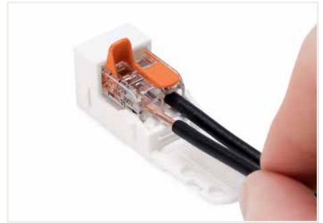
Inserting a conductor.
