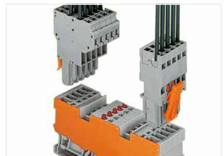
2-pin LED carrier terminal block; with two jumper positions 2-conductor female plug 1-conductor female plug; straight
