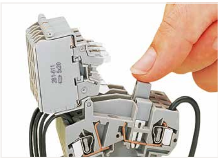
Commoning Distributing current to several fuse-protected circuits via insulated push-in type jumpers.
