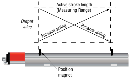
Figure 1. Analog Output signals
