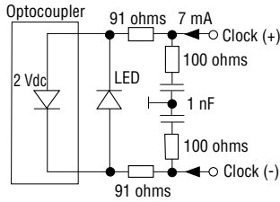
Figure 1. Sensor input
