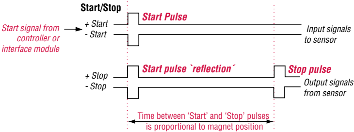
Figure 2. Start/Stop output signals (RS-422 differential pairs)
