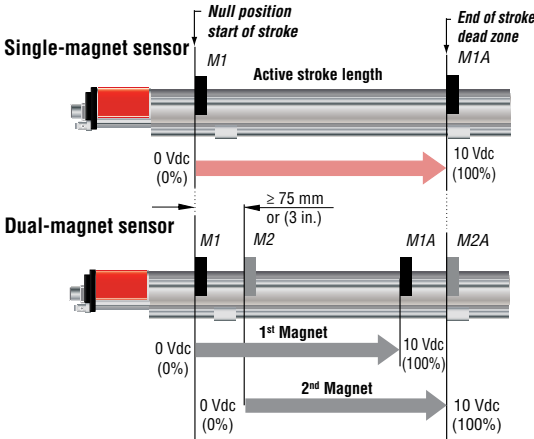
Figure 3. Single and dual magnet measurements
