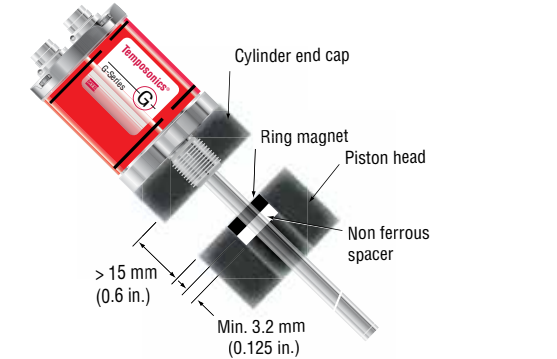
Figure 5. Models GT2/GT3 rod-style mounting
