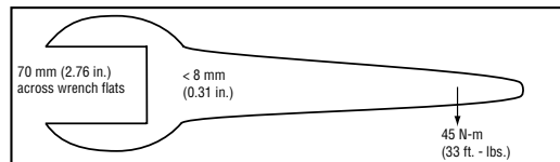
Figure 5. Basic wrench
