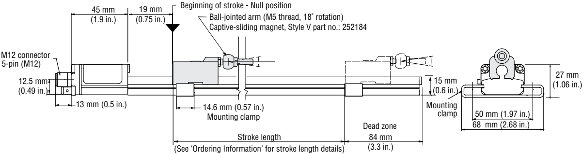
Figure 3. E-Series model EL sensor dimension reference (Shown with Style V captive-sliding magnet)
