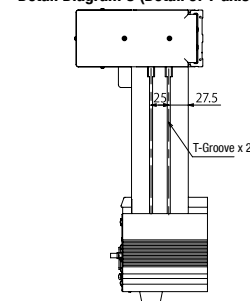
X View (T-Groove on the Side of the Main Unit)
