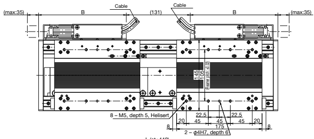
Detail view of base mount (S-1)
