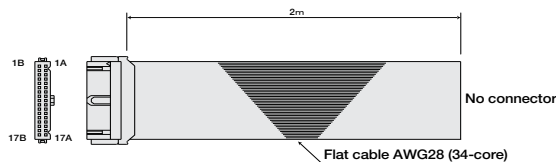
Flat cable AWG28 (34-core)
