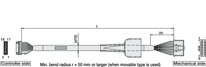
Min. bend radius r = 50 mm or larger (when movable type is used) * Only the robot cable is to be used in a cable track.
