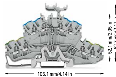
4-conductor double-deck terminal block; ground conductor/through terminal block; with marker carrier; gray
