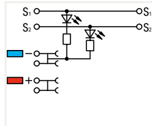
3-conductor sensor terminal block; yellow LED; for PNP (high-side) switching sensors
