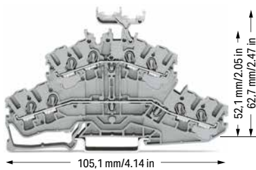
4-conductor double-deck terminal block; through/through terminal block; with marker carrier; gray
