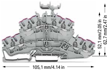
4-conductor double-deck terminal block; 8-conductor through terminal block; with marker carrier; internally commoned; violet conductor entry; gray
