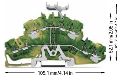
4-conductor double-deck terminal block; 8-conductor ground terminal block; with marker carrier; internally commoned; green-yellow
