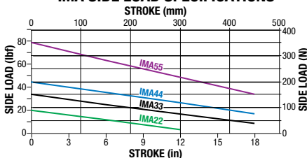
IMA SIDE LOAD SPECIFICATIONS
