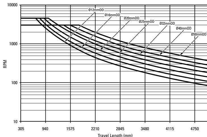
Speed vs Length (Metric Series) BK-BK, FK-FK, MK-BK, WK-WK
