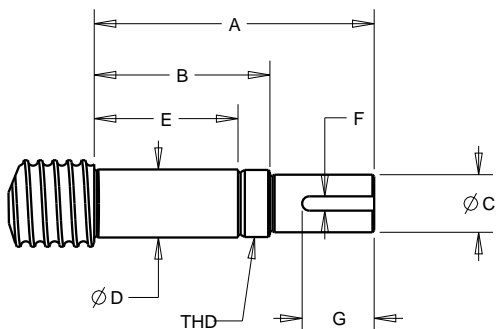
TYPE WK, REQUIRED FOR WK SUPPORT
