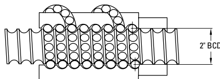
Ball Circle Diameter (BCD)
