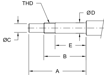
TYPE MK, REQUIRED FOR MK SUPPORT
