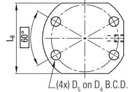
HOLE PATTERN 0 ≤ 12 mm ONLY
