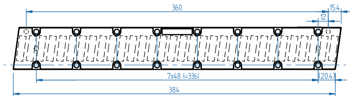
TM 384mm
