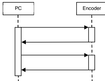
Figure 3: Communication cycle.
