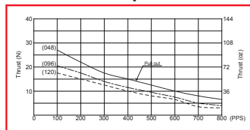
Unipolar Constant Voltage 48C4 Torque Curve
