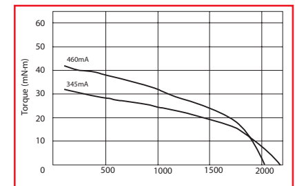
Unipolar Constant Current (48071)
