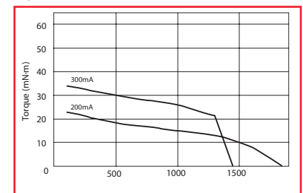
Bipolar Constant Current (48271)
