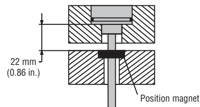
Figure 4. Model MS installation in non-magnetic material (without a non-ferrous magnet spacer).
