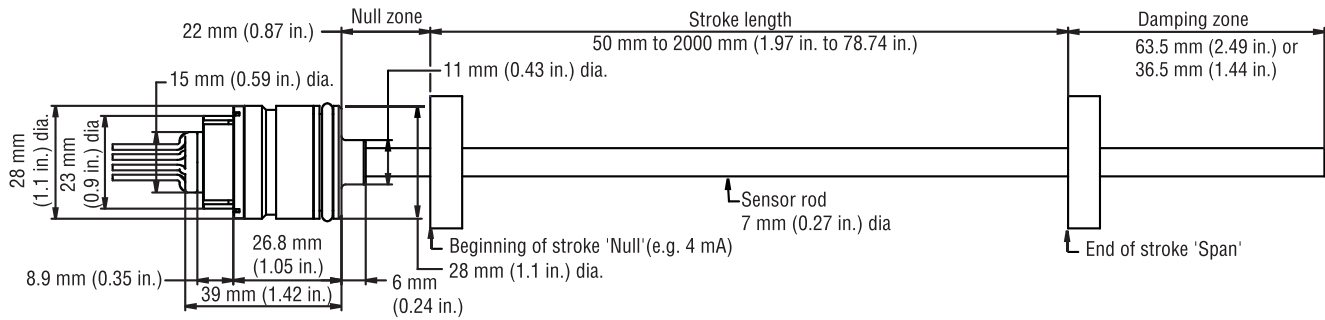
Figure 1. MH-Series Model MS rod-style sensor dimension reference
