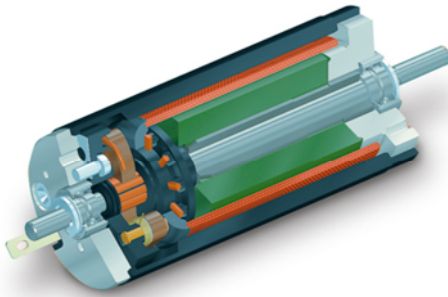
Figure 3: maxon motor RE 25, Ø 25 mm, graphite brushes, 20 Watt
