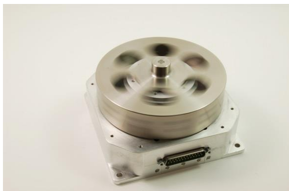
maxon motors drive the reaction wheels that control the inclination of the satellite. © Clyde Space
