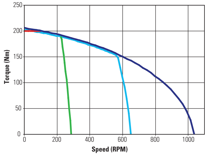
KBM(S)-88X01 ContinuousTorque
