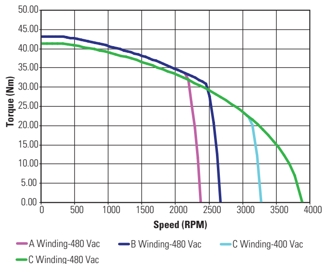
KBM(S)-45X02 ContinuousTorque
