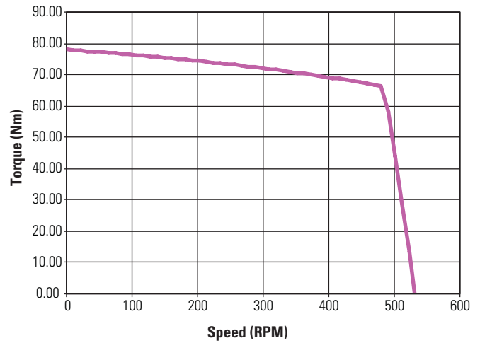
KBM(S)-79X02 ContinuousTorque
