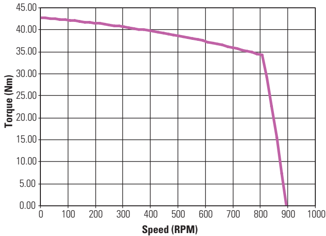
KBM(S)-79X01 ContinuousTorque
