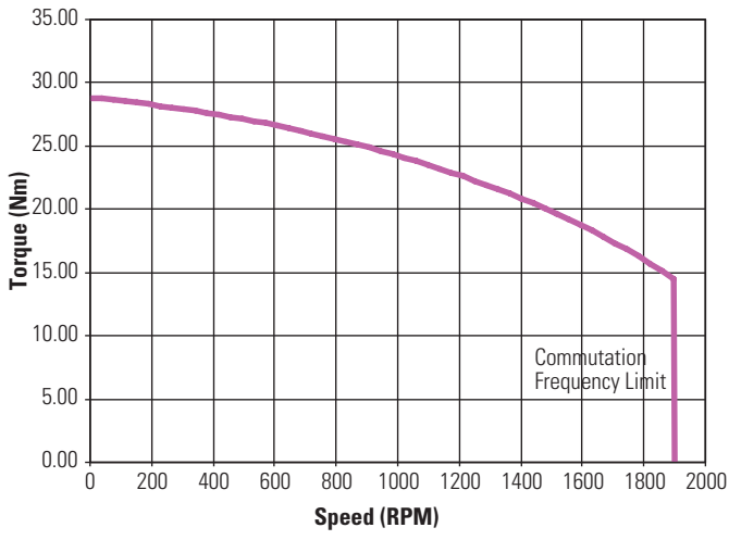
KBM(S)-60X00 ContinuousTorque
