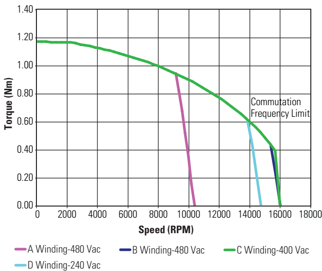
KBM(S)-10X03 ContinuousTorque
