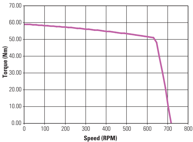
KBM(S)-57X03 ContinuousTorque
