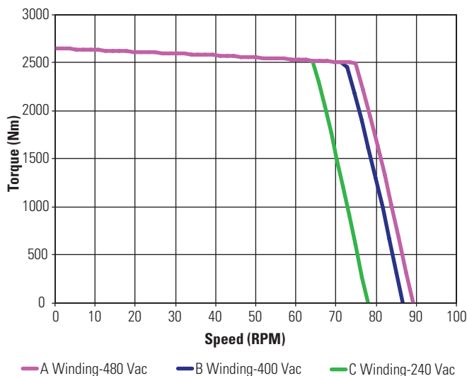
KBM(S)-260X02 ContinuousTorque
