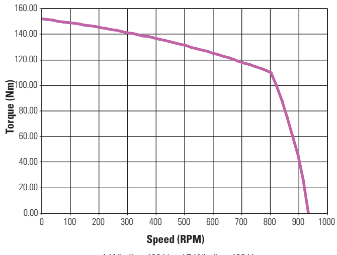
KBM(S)-60X03 ContinuousTorque
