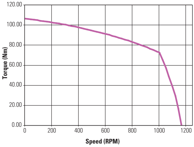
KBM(S)-60X02 ContinuousTorque
