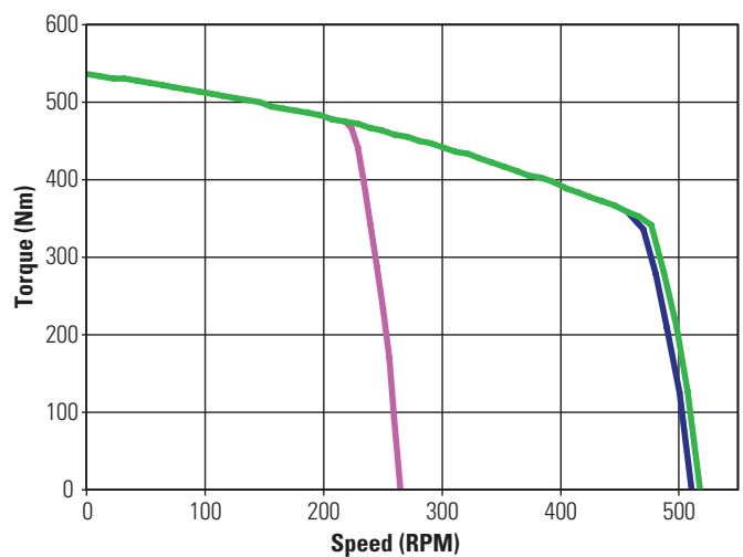
KBM(S)-88X03 ContinuousTorque
