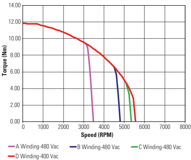
KBM(S)-25X03 ContinuousTorque
