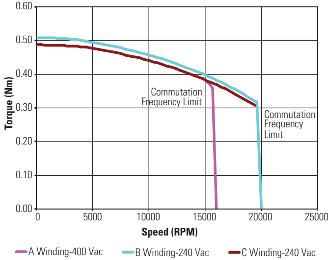
KBM(S)-10X01 ContinuousTorque
