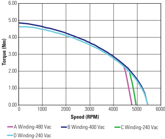
KBM(S)-25X01 ContinuousTorque
