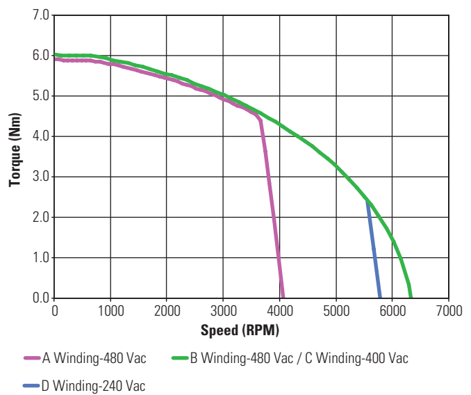
KBM(S)-17X04 ContinuousTorque
