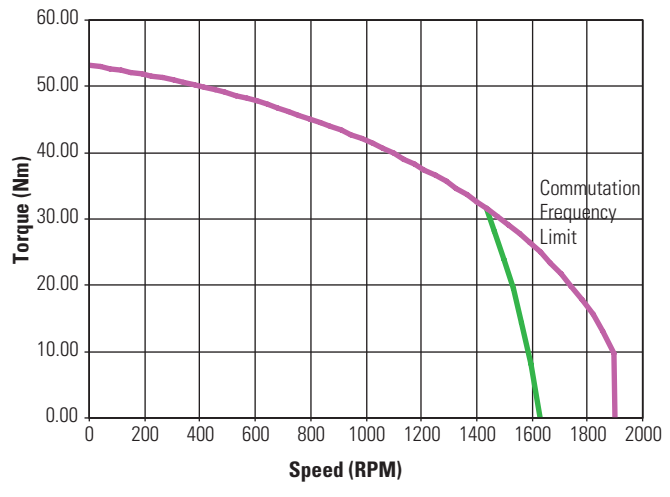
KBM(S)-60X01 ContinuousTorque
