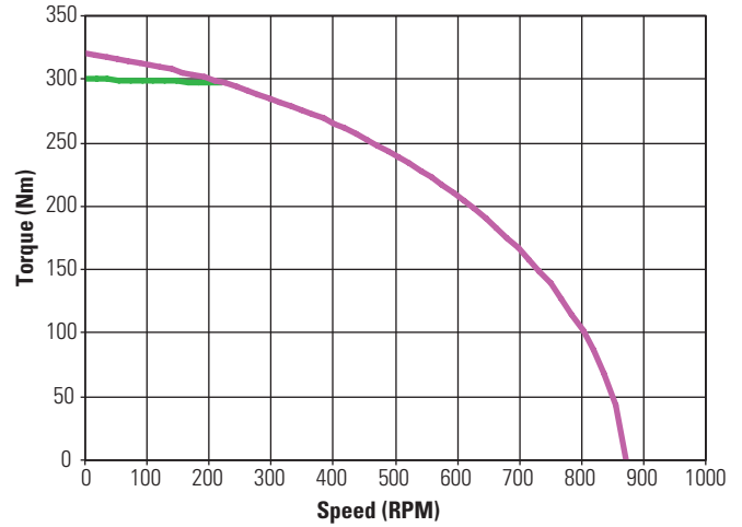
KBM(S)-118X01 ContinuousTorque
