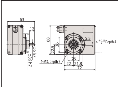
RCP2-RTCS/RTCSL Combination Drawing
