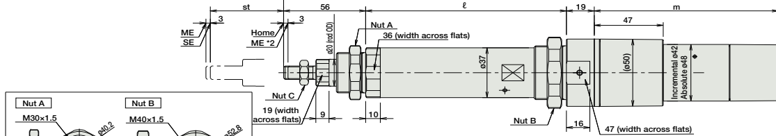
RCA-RA4C (without brake)
