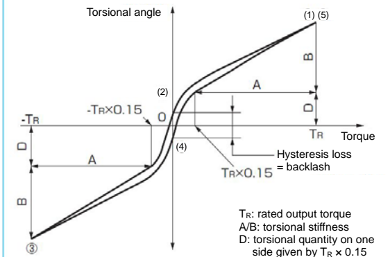
Fig. 1 Torque vs. torsional angle diagram
