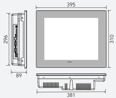
Panel cut
