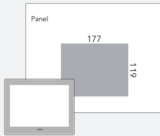
Panel cut
