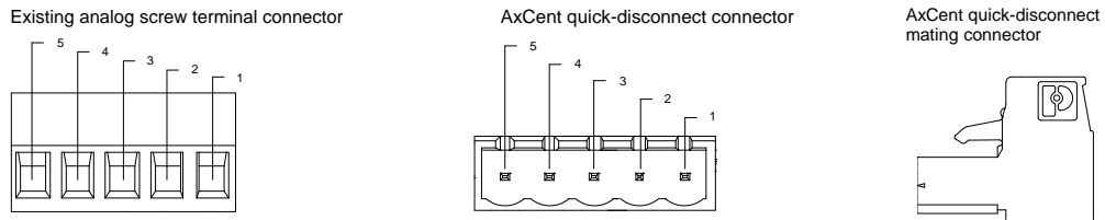
Figure 5 P2 Connector – Existing Analog and AxCent Drives
