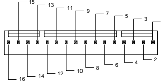
Figure 16 P1 Connector – Existing Analog and AxCent Drives
