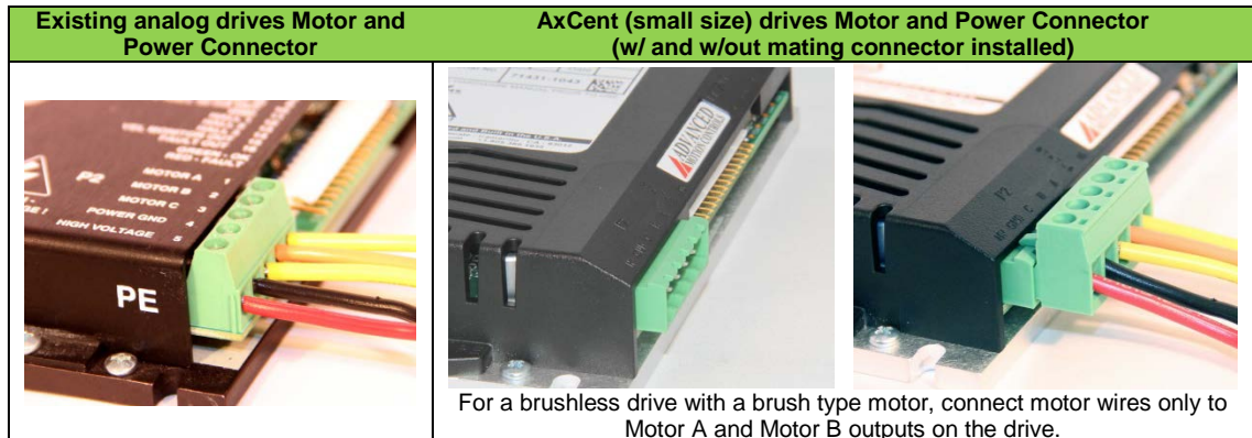
Figure 6 Motor and Power Connector
