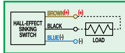
HALL-EFFECT, SINKING, NPN
