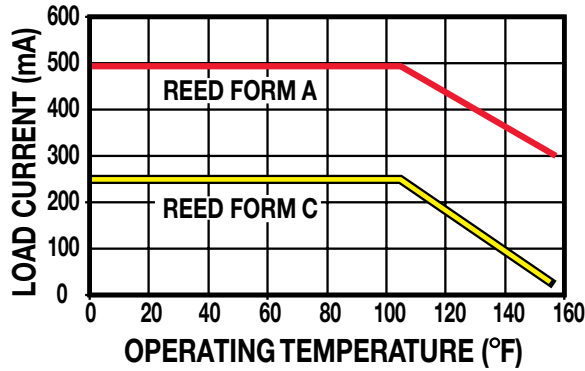
TEMP. vs CURRENT, DC REED
