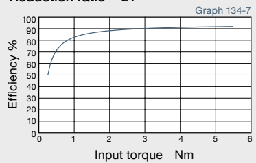
Reduction ratio = 21
