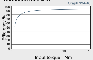
Reduction ratio = 31
