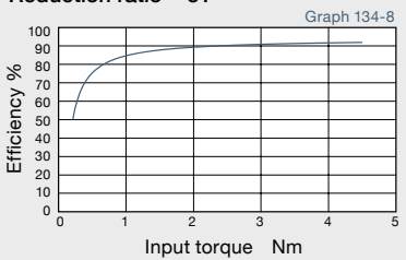
Reduction ratio = 31
