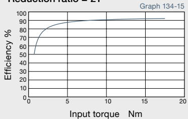
Reduction ratio = 21
